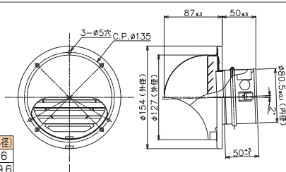
TZ-FBC80NKP/100NKP
