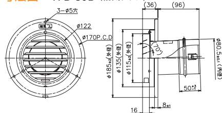
TFB-80B/100B(分離型)
