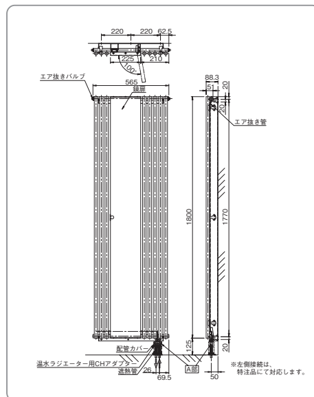
寸法図(ZIR-0803AWN-1805M/DM)
