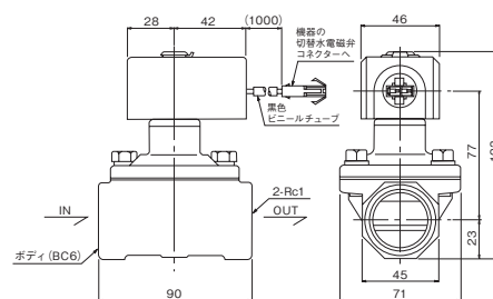
CCP水電磁弁3
